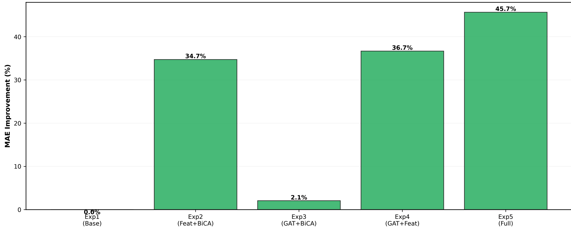
Component Contribution to MAE Reduction (Relative to Baseline)
